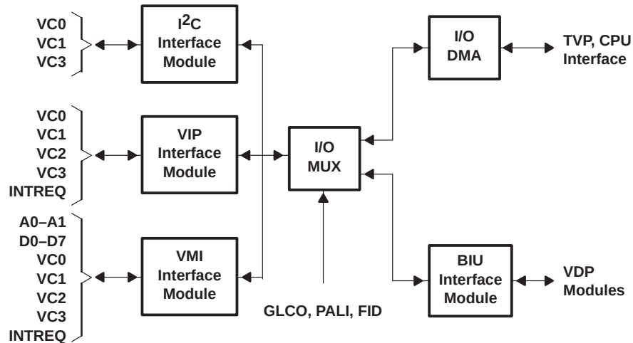
Figure 2-19. Host Interface
