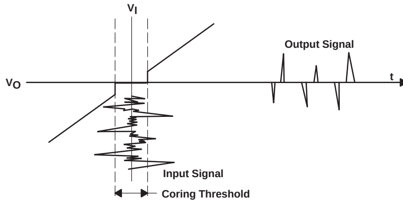
Figure 2-9. Transfer Curve of Coring Circuit
