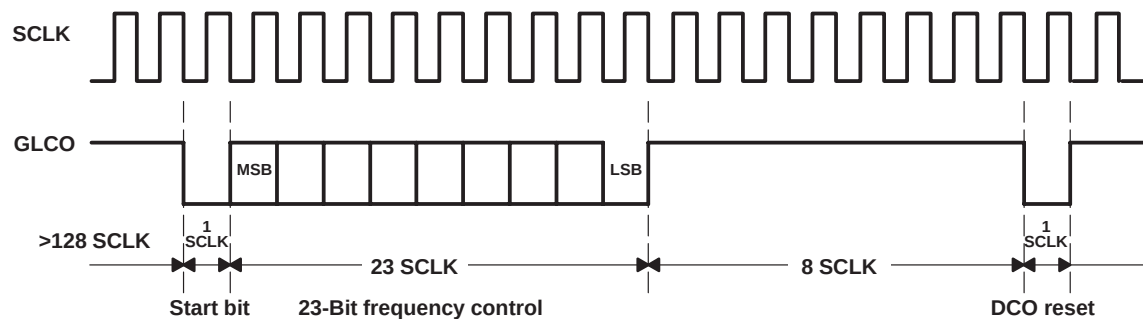
Figure 2–30. GLCO Timing
