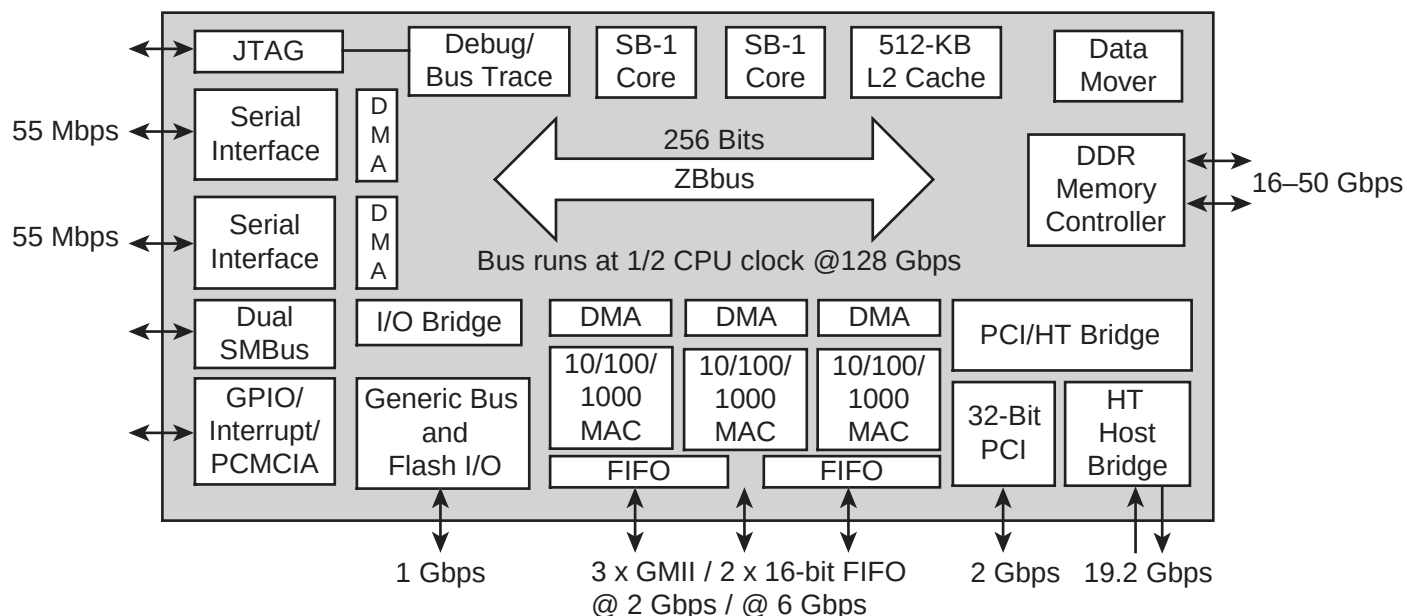
BCM1250 Block Diagram
