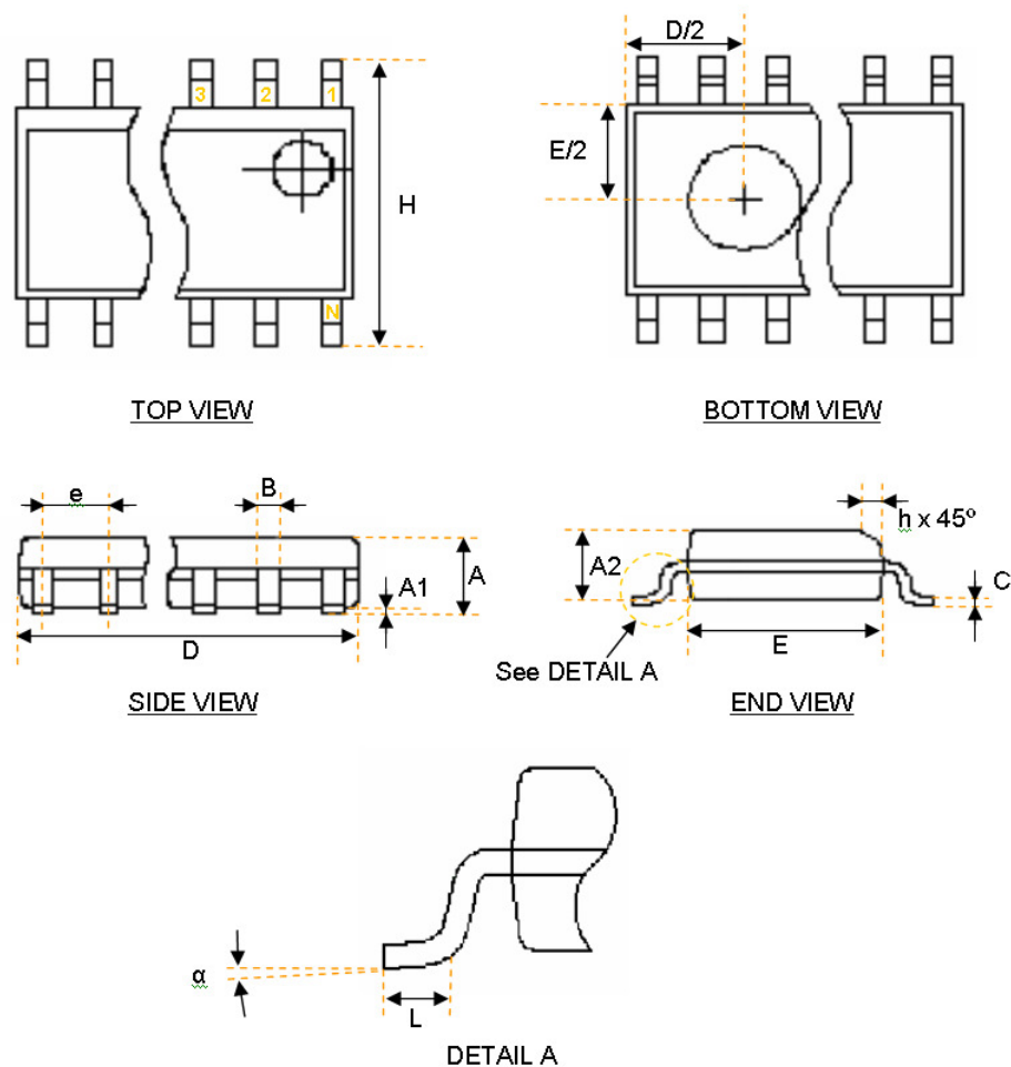
Figure 11: Package information drawing
