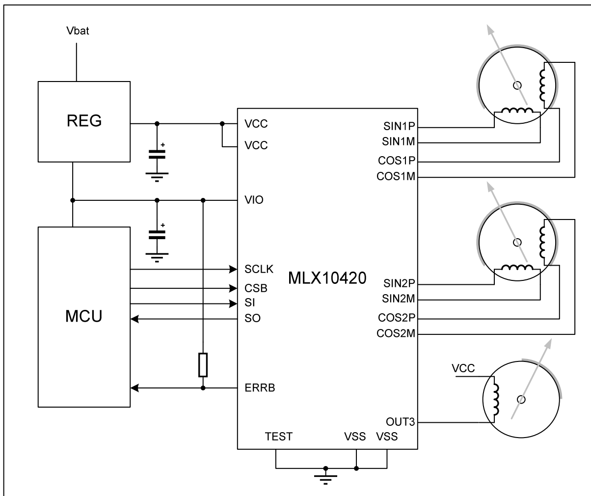
Figure 10: Typical application diagram
