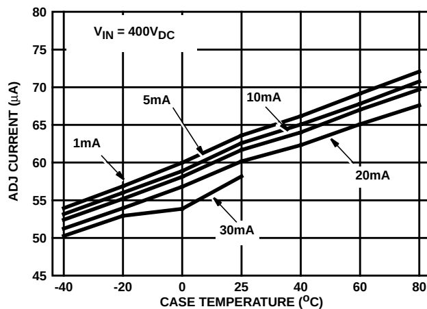
FIGURE 35. I_{ADJ} vs TEMPERATURE
