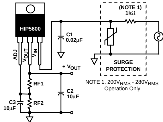
FIGURE 13. AC/DC CONVERTER
