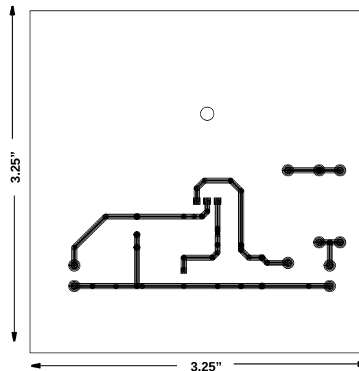
FIGURE 40. EVALUATION BOARD METAL MASK (BOTTOM)
