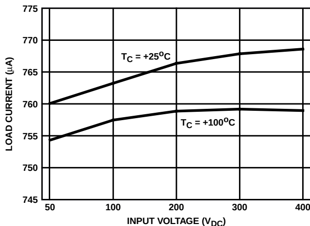
FIGURE 36. MINIMUM LOAD CURRENT vs V_{IN}
