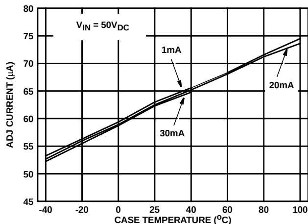
FIGURE 34. I_{ADJ} vs TEMPERATURE
