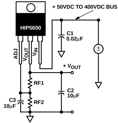
FIGURE 12. DC/DC CONVERTER
