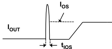
Figure 27. Output Short Circuit Parameters
