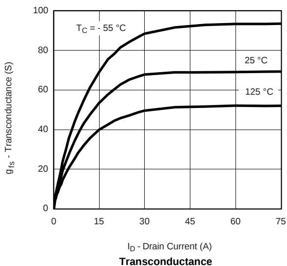
Transconductance
