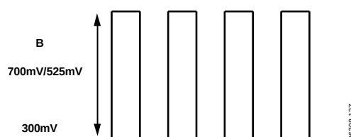
Figure 125. HD RGB Output Levels—RGB Sync Disabled
