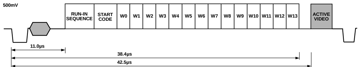
Figure 97. WSS Waveform Diagram
