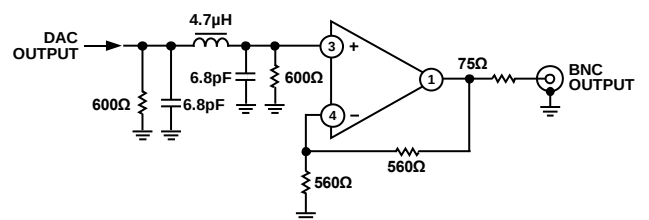
Figure 84. Example of Output Filter for ED, 8x Oversampling
