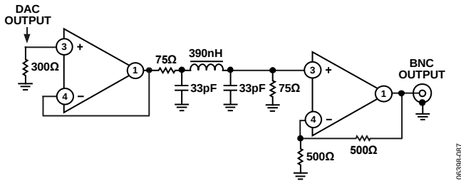
Figure 85. Example of Output Filter for HD, 4x Oversampling
