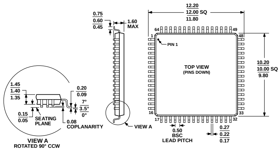
COMPLIANT TO JEDEC STANDARDS MS-026-BCD Figure 139. 64-Lead Low Profile Quad Flat Package [LQFP] (ST-64-2) Dimensions shown in millimeters
