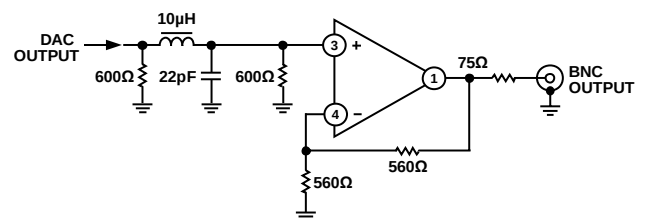
Figure 83. Example of Output Filter for SD, 16x Oversampling
