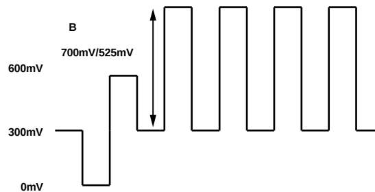
Figure 126. HD RGB Output Levels—RGB Sync Enabled
