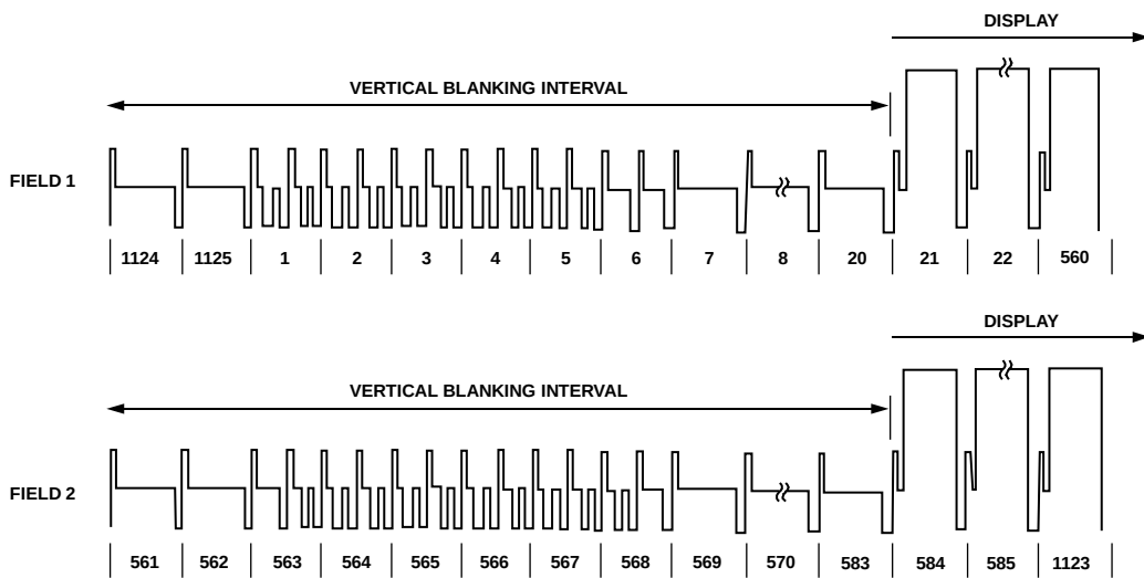
Figure 138. SMPTE 274M (1080i)
