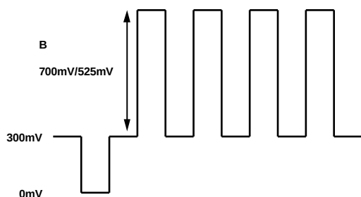
Figure 124. SD/ED RGB Output Levels—RGB Sync Enabled
