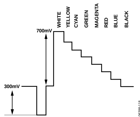
Figure 116. Y Levels—PAL
