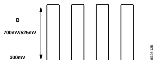
Figure 123. SD/ED RGB Output Levels—RGB Sync Disabled
