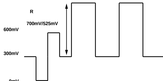
Figure 125. HD RGB Output Levels—RGB Sync Disabled
