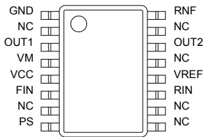
Fig.30 BA6285FS (SSOP-A16)
