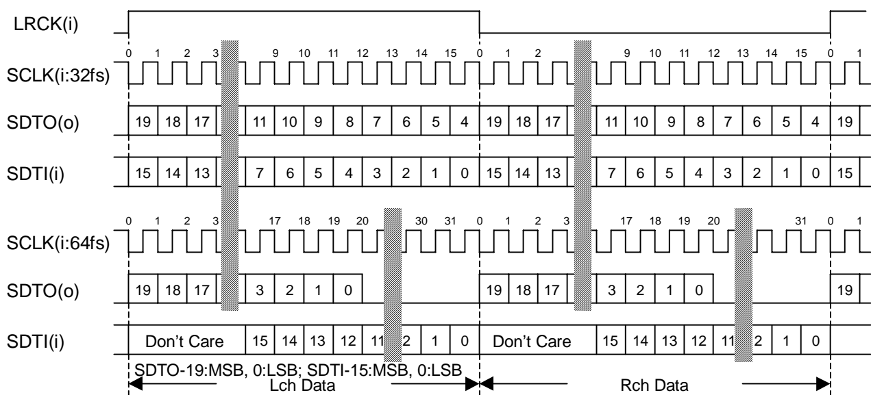
Figure 1. Mode 0 Timing
