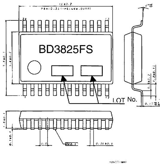
Figure - 1 PACKAGE (SSOP-A24)
