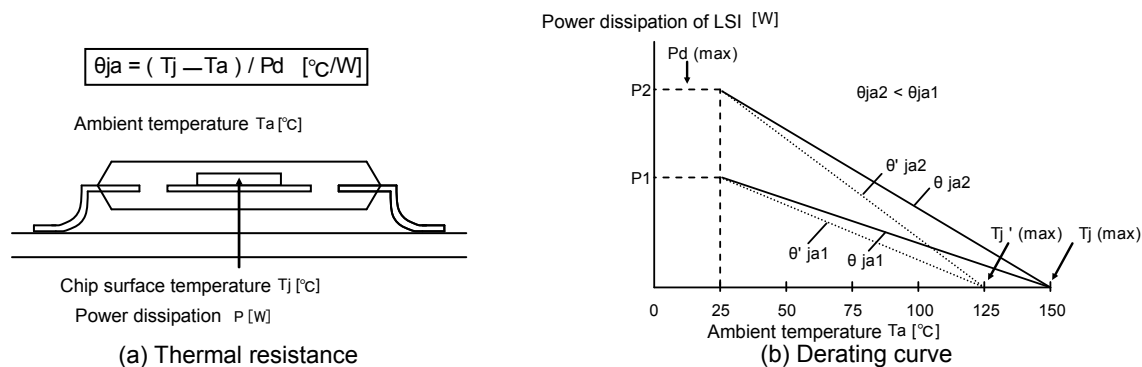
Fig. 124 Thermal resistance and derating curve
