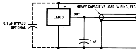
Figure 6. LM60 with Filter for Noisy Environment
