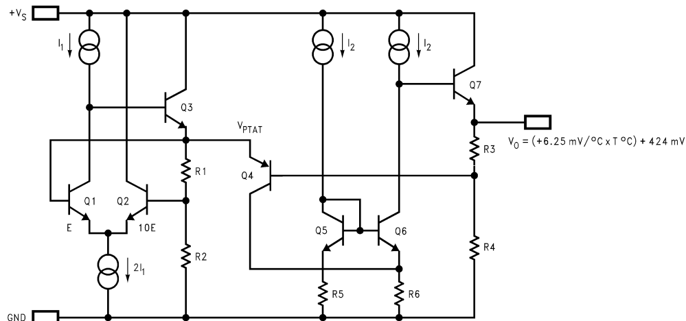
Figure 7. Simplified Schematic
