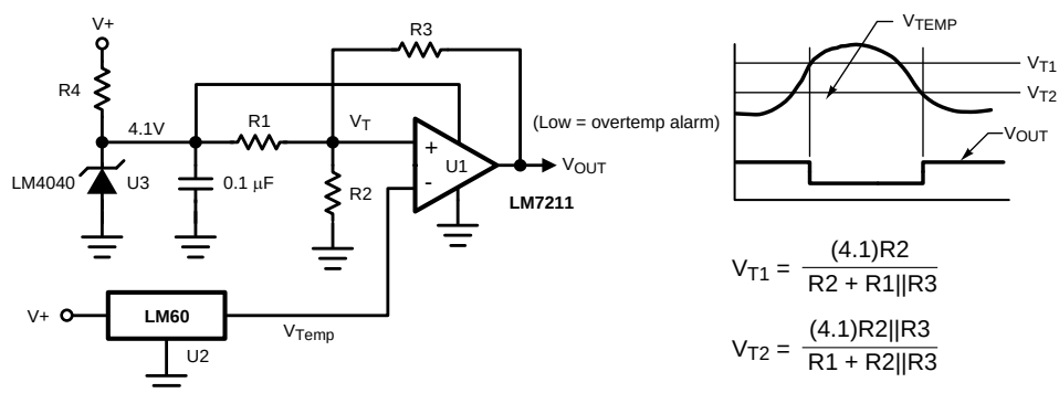
Figure 8. Centigrade Thermostat
