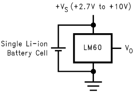
Figure 1. Full-Range Centigrade Temperature Sensor (–40°C to +125°C) Operating from a Single Li-Ion Battery Cell
