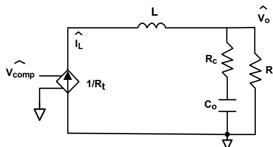
FIGURE 36. POWER TRAIN SMALL SIGNAL MODEL
