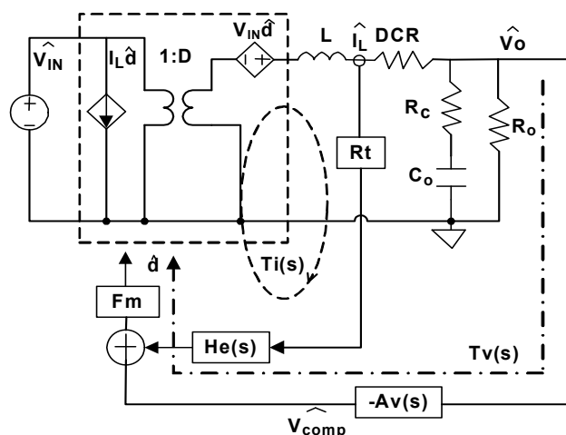
FIGURE 35. SMALL SIGNAL MODEL OF SYNCHRONOUS BUCK REGULATOR
