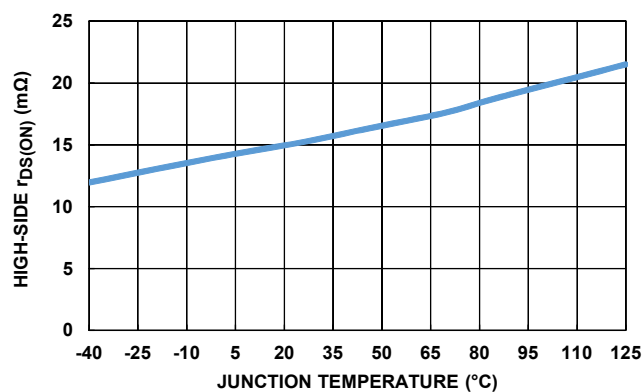
FIGURE 27. HIGH-SIDE r DS(ON) vs TEMPERATURE
