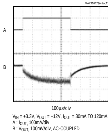
LOAD-TRANSIENT RESPONSE
