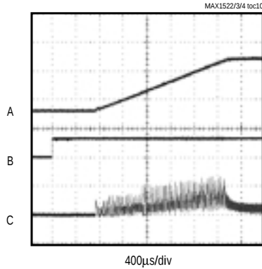
SOFT-START RESPONSE
