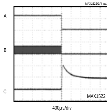
FAULT-DETECTION RESPONSE
