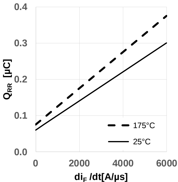
Figure 19 Typical reverse recovery charge as a function of diode current slope (Q_{rr} = f(di_i/dt), V_{DD} = 800V, V_{GS} = 0V/18V, I_D = 6A, \text{ind. load, test circuit in Fig. E, body diode at } V_{GS} = 0V)
