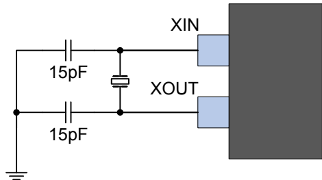
Figure 49-7. Crystal Oscillator Schematic
