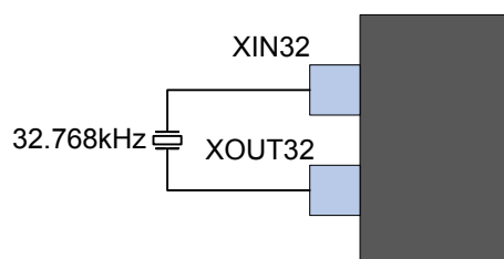
Figure 49-8. External Real Time Oscillator without Load Capacitor
