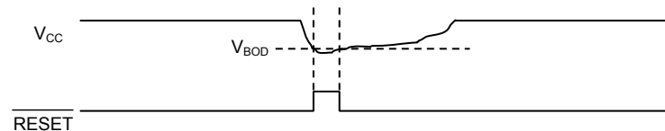
Figure 45-3. BODVDD Hysteresis ON
