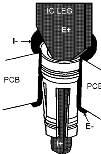
Figure 3 Low level Contact Resistance Measurement Points
