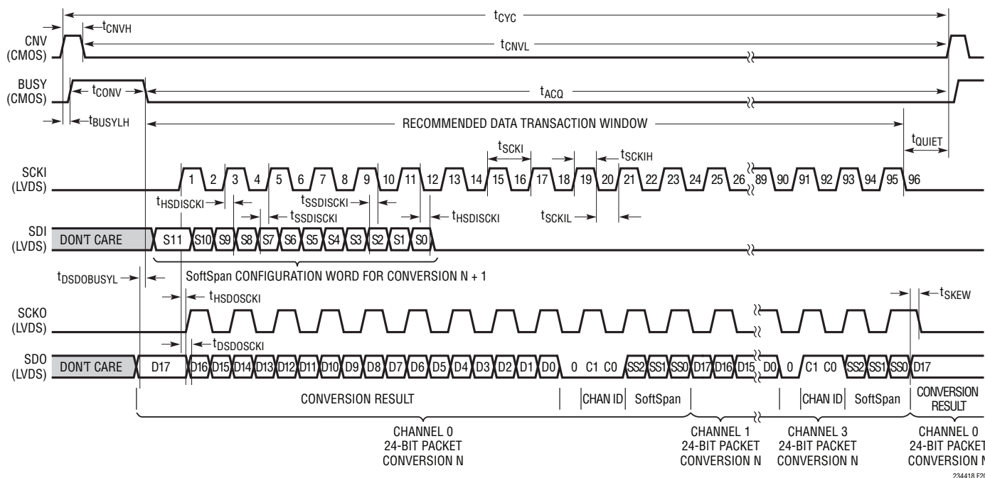
Figure 20. Serial LVDS I/O Mode
