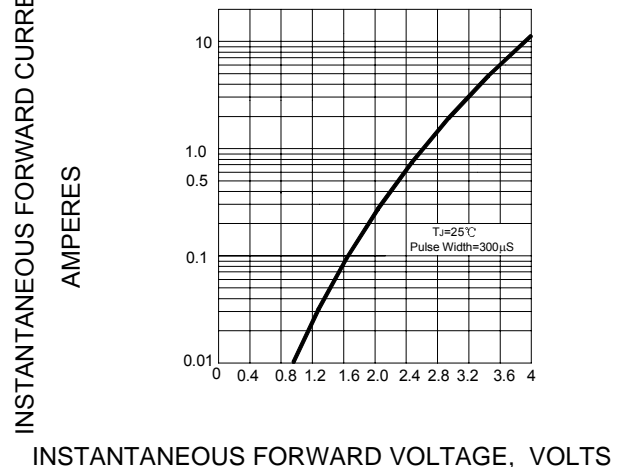
FIG.5 -- TYPICAL FORWARD CHARACTERISTIC
