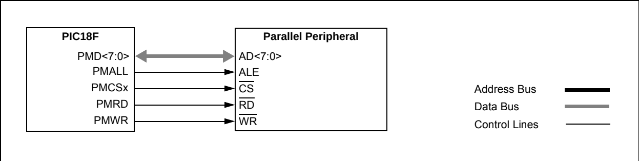
FIGURE 11-29: EXAMPLE OF AN 8-BIT MULTIPLEXED ADDRESS AND DATA APPLICATION
