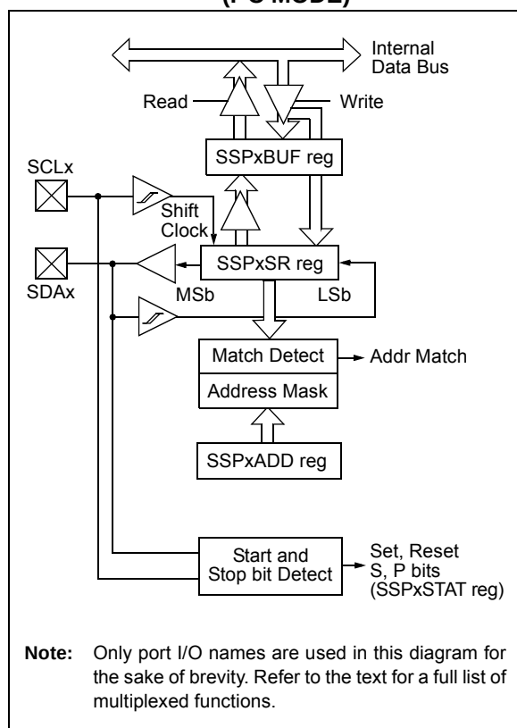
FIGURE 20-7: MSSPx BLOCK DIAGRAM (I 2 C MODE)
