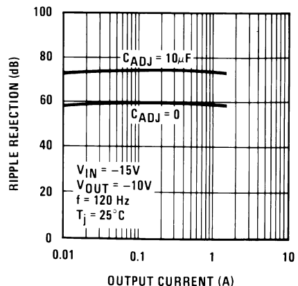
Figure 9. Ripple Rejection
