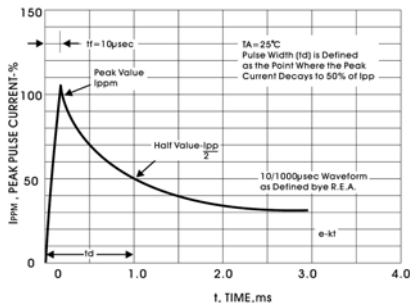
FIGURE 3-PULSE WAVEFORM
