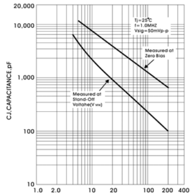
FIGURE 4 TYPICAL CAPACITANCE VS STAND-OFF VOLTAGE
