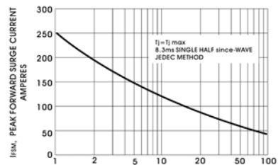
FIG. 6-MAXIMUM NON-REPETITIVE PEAK FORWARD SURGE CURRENT UNIDIRECTIONAL
