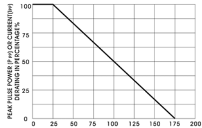
FIGURE 2-DERATING CURVE
