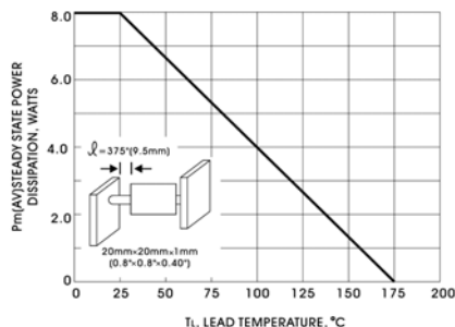
FIG. 5-STEADY STATE POWER DERATING CURVE
