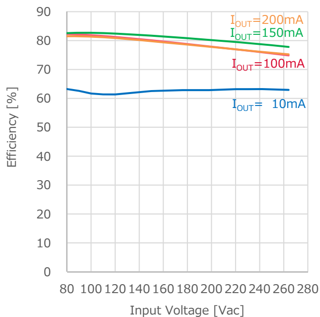
Figure 11. LINE Regulation ( I_{OUT} vs. Efficiency)
