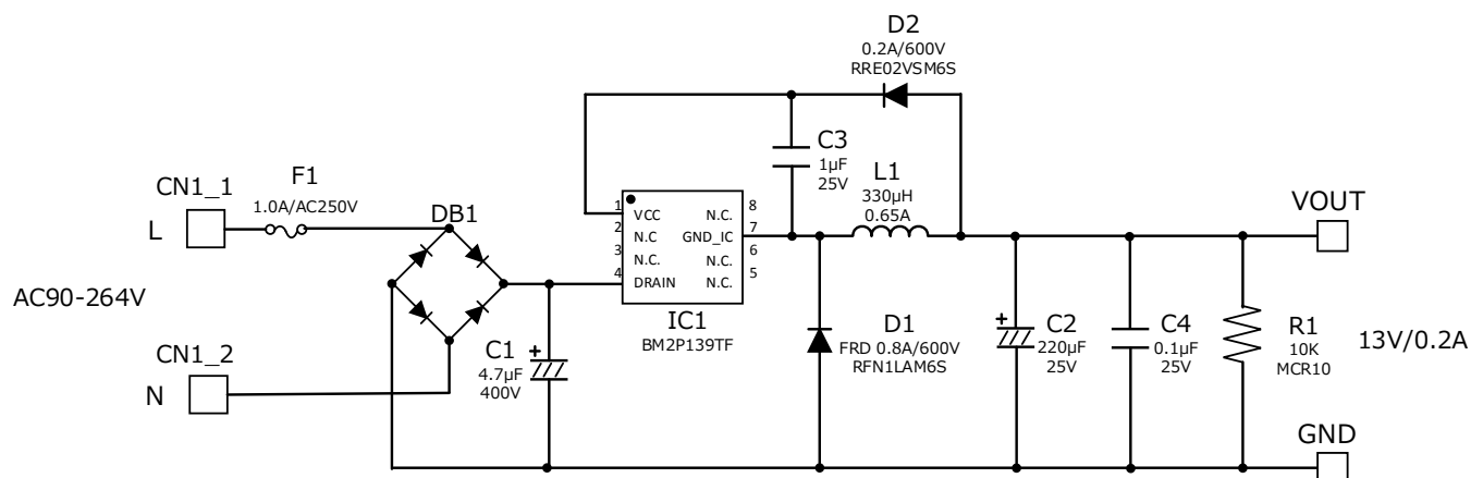
Figure 3. BM2P139TF-EVK-001 Schematics
