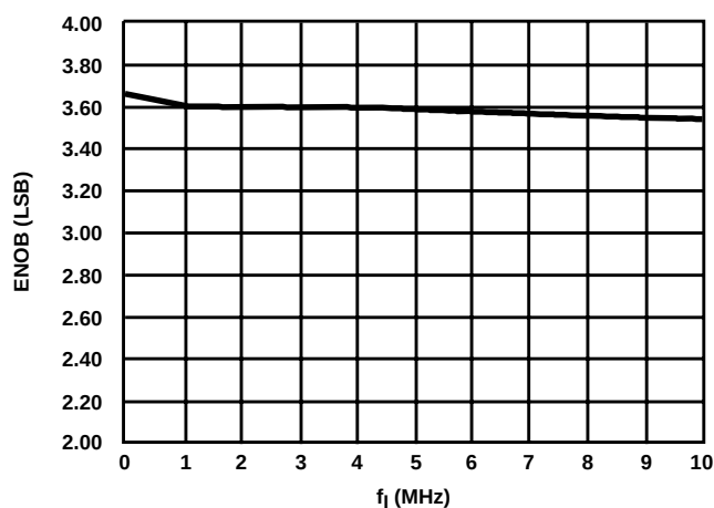
FIGURE 10. EFFECTIVE BITS vs INPUT FREQUENCY
