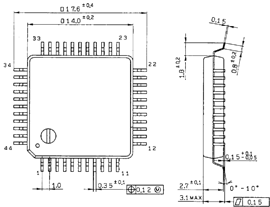
44pin QFP (Plastic) 1.1g
