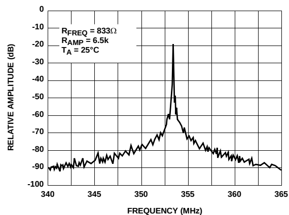
FIGURE 14. OUTPUT SPECTRUM - WIDEBAND
