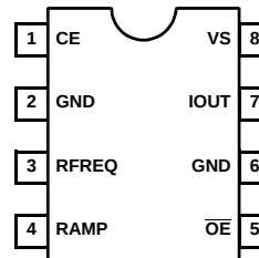
EL6201 (8-PIN MSOP) TOP VIEW
