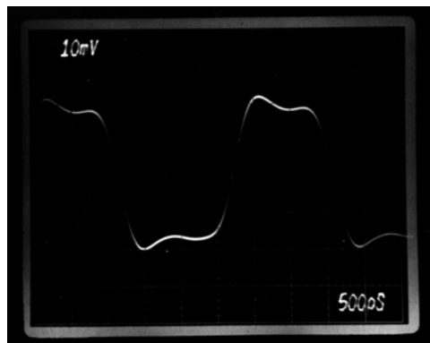
FIGURE 21. OUTPUT CURRENT WAVEFORM - 1GHz BANDWIDTH
