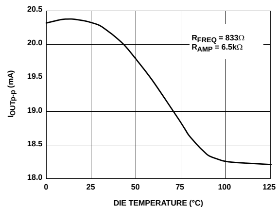
FIGURE 16. I_{OUTp-p} vs DIE TEMPERATURE
