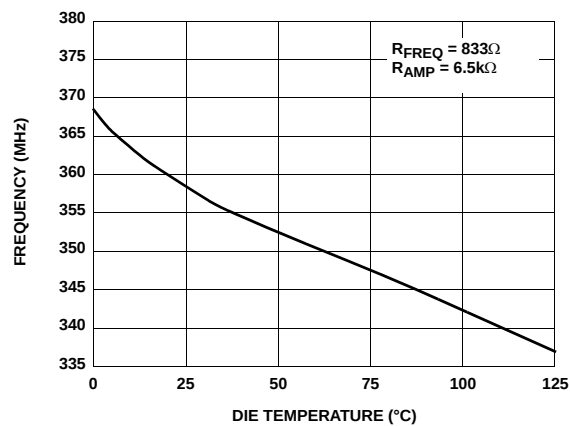
FIGURE 18. FREQUENCY vs DIE TEMPERATURE
