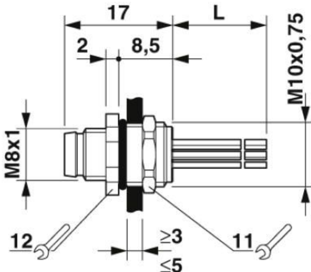
Dimensional drawing
