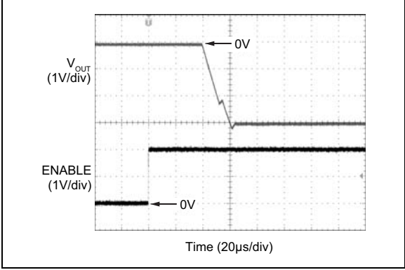
FIGURE 2-17: Positive Enable Transient.
