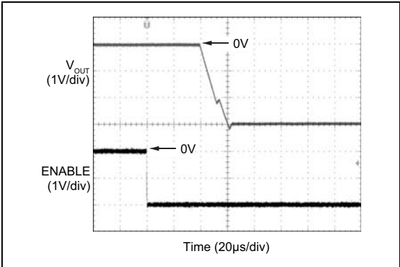
FIGURE 2-16: Negative Enable Transient.
