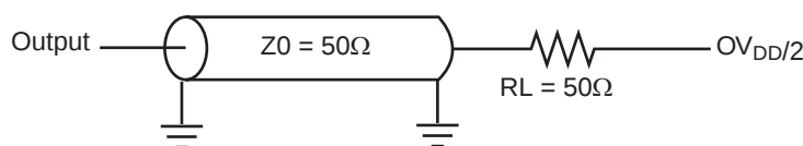
Figure 10. AC Test Load for the 60x Interface
