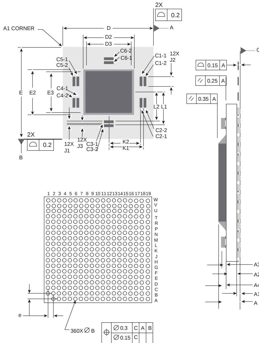
Figure 25. Mechanical Dimensions and Bottom Surface Nomenclature of the 360-ball CBGA Package
