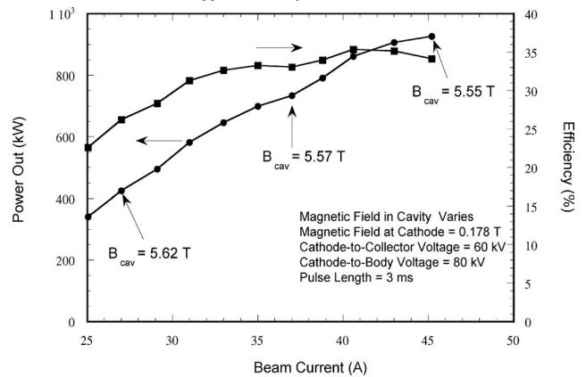
Power & Efficiency vs. Beam Current
