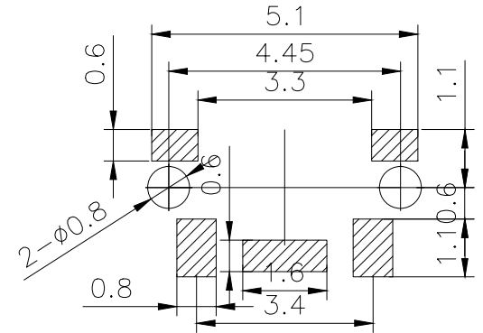
PCB. WELDING DRAWING
