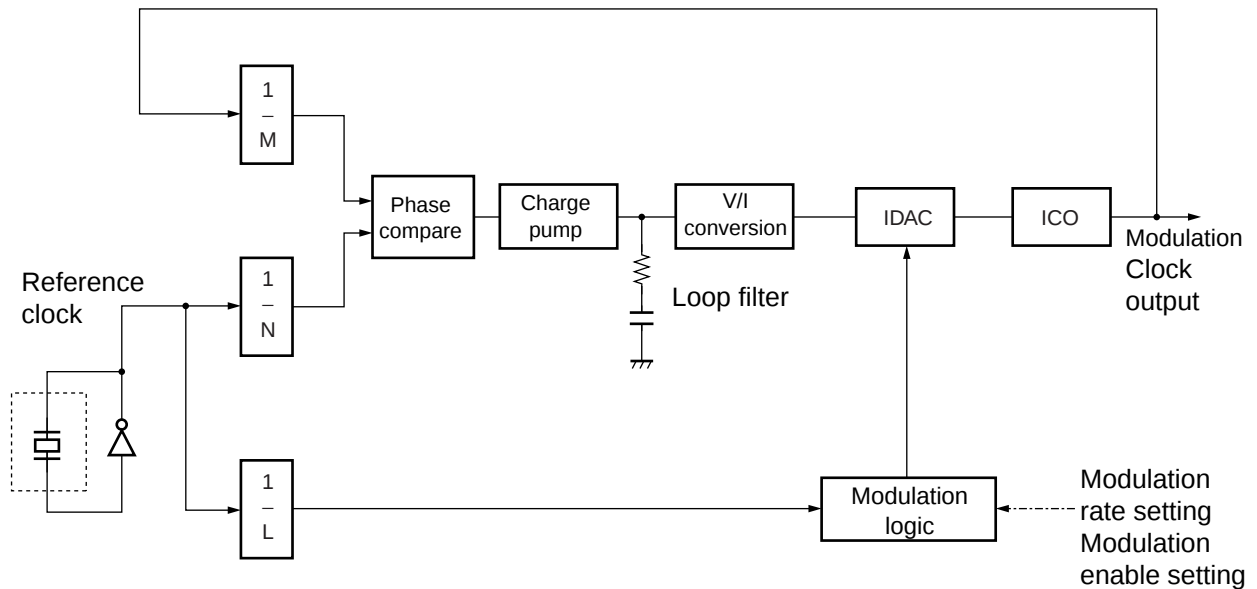
MB88154 PLL block
