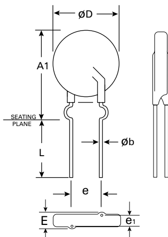
Outer Crimped Lead Option
