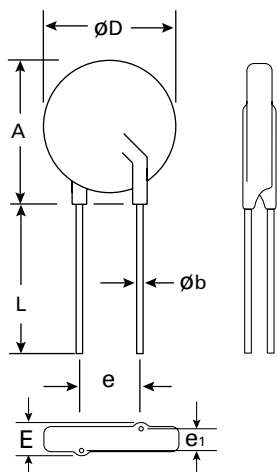
Straight Lead Option
