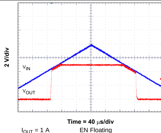
Figure 48. Low Dropout Operation
