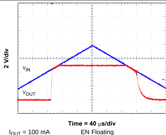
Figure 47. Low Dropout Operation
