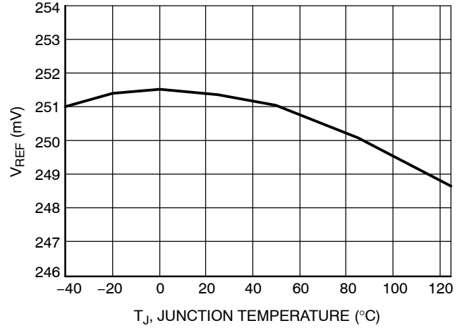
Figure 16. V REF vs. Junction Temperature
