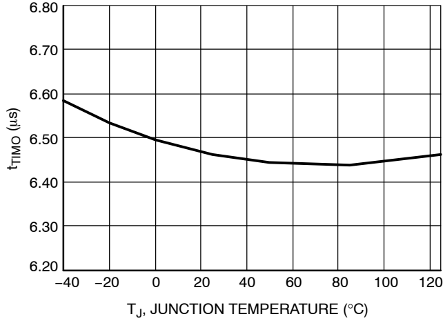
Figure 15. t TMO vs. Junction Temperature
