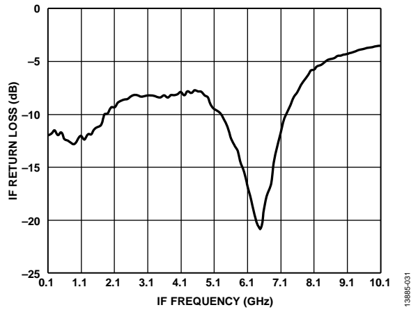
Figure 30. IF Return Loss vs. IF Frequency LO = 13 dBm at 17 GHz
