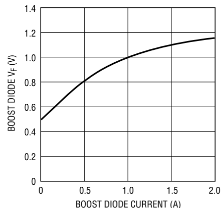
Boost Diode
