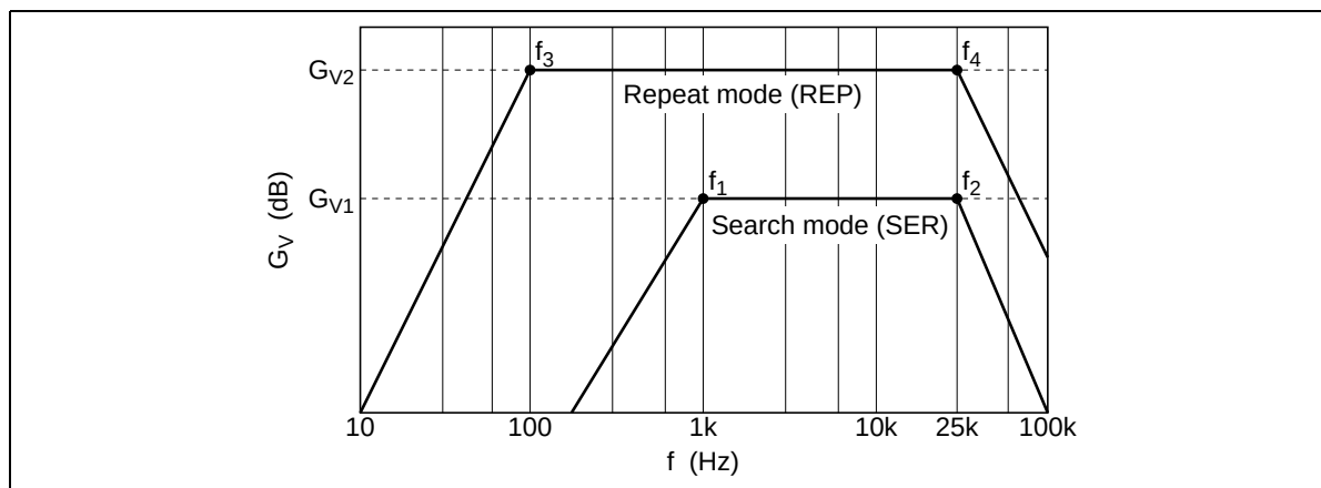
Figure 5 Frequency Response
