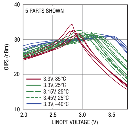
Output IP3 vs LINOPT Voltage ( f_{LO} = 450MHz , P_{LOM} = 0dBm )
