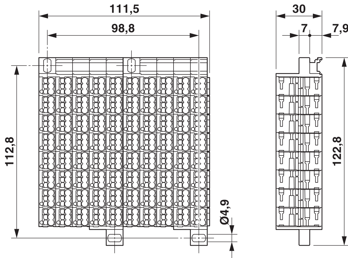
Dimensional drawing
