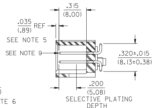
SECTION J-J
