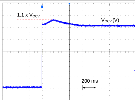
图 30. Typical V_{OUT} Start Up at No Load
