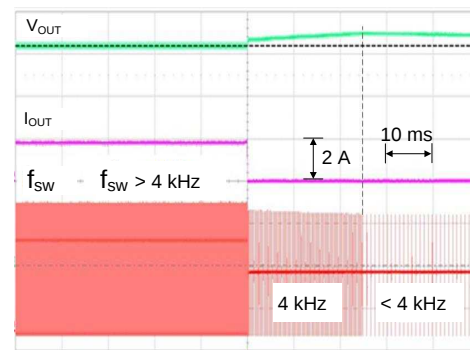
图 29. Response to Load Step-Down
