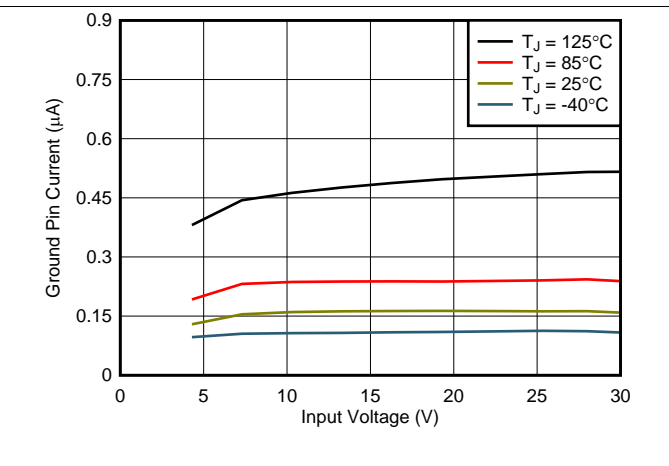
Figure 22. 3.3-V Shutdown Current vs V_{IN} and Temperature
