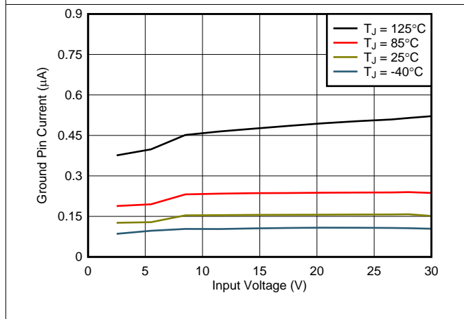
Figure 21. 1.2-V Shutdown Current vs V_{IN} and Temperature
