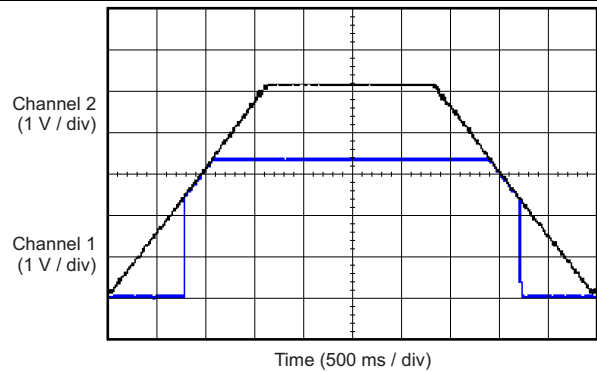
Channel 1 = V_{IN} , channel 2 = V_{OUT} , I_{OUT} = 3\text{ mA} , TPS70633
