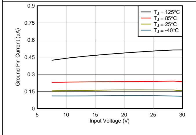
Figure 23. 6.5-V Shutdown Current vs V_{IN} and Temperature
