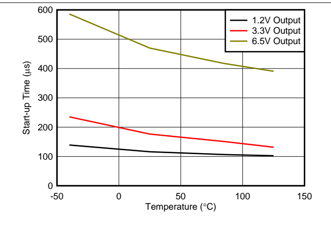
Figure 24. Start-Up Time vs Temperature
