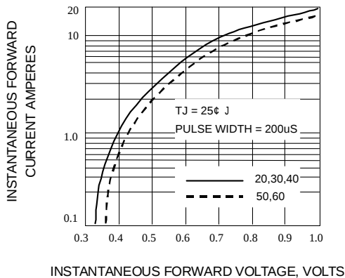
Fig. 4-TYPICAL FORWARD CHARACTERISTICS
