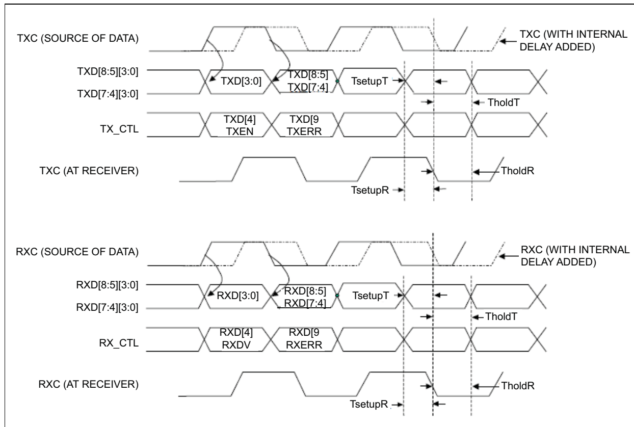
FIGURE 7-2: RGMII V2.0 SPECIFICATION
