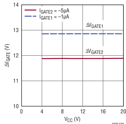
MOSFET Gate Drive vs V_{CC} Voltage
