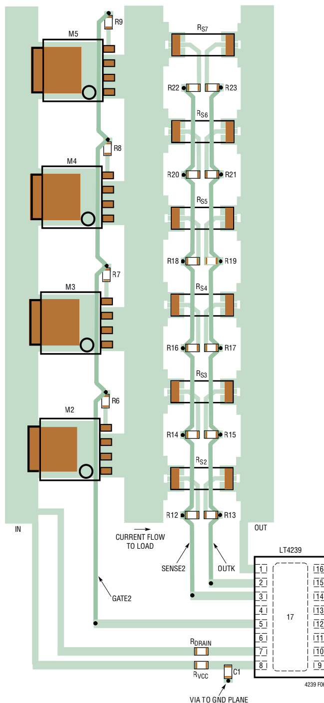
Figure 6. Recommended Layout
