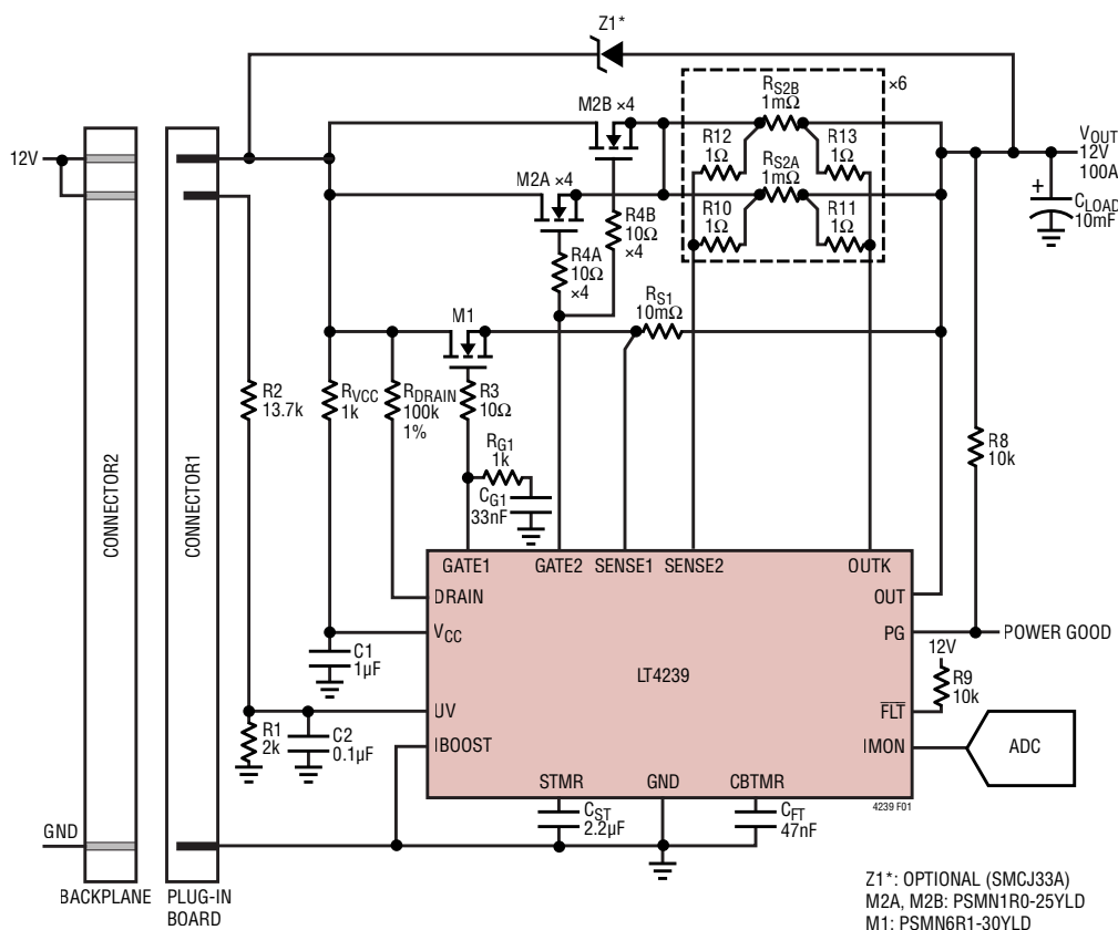
Figure 1. Typical Application
