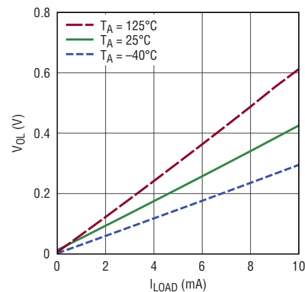
FLT and PG Output Low Voltage vs Load Current
