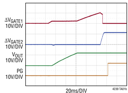
Start-Up Waveforms
