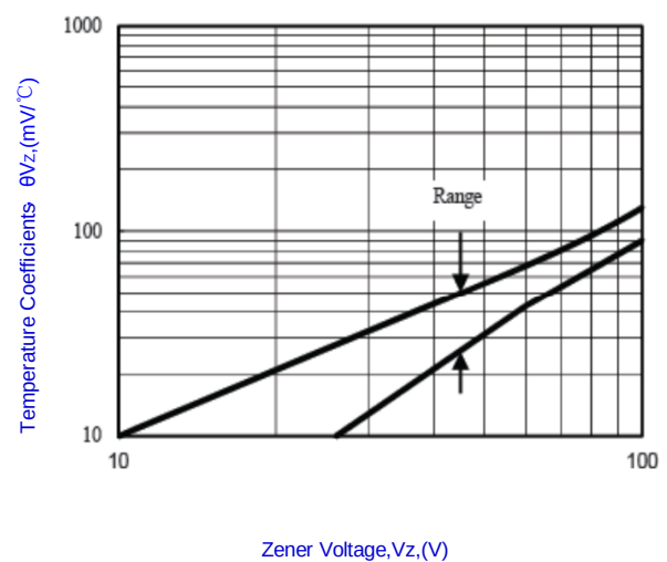
Fig.2- Temperature Coefficients v.s. Zener Voltage
