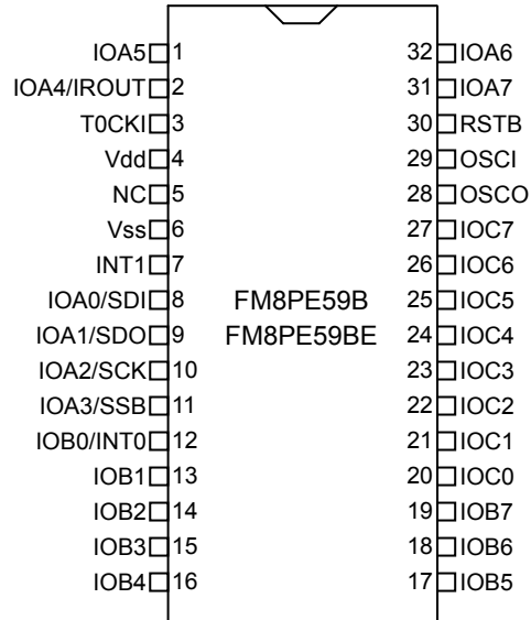
PDIP, SOP
