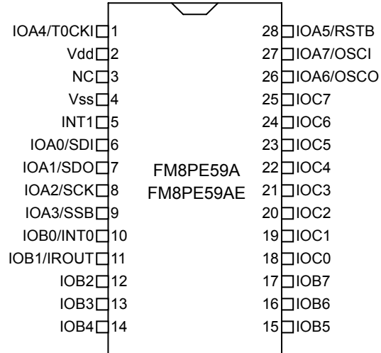
PDIP, SOP
