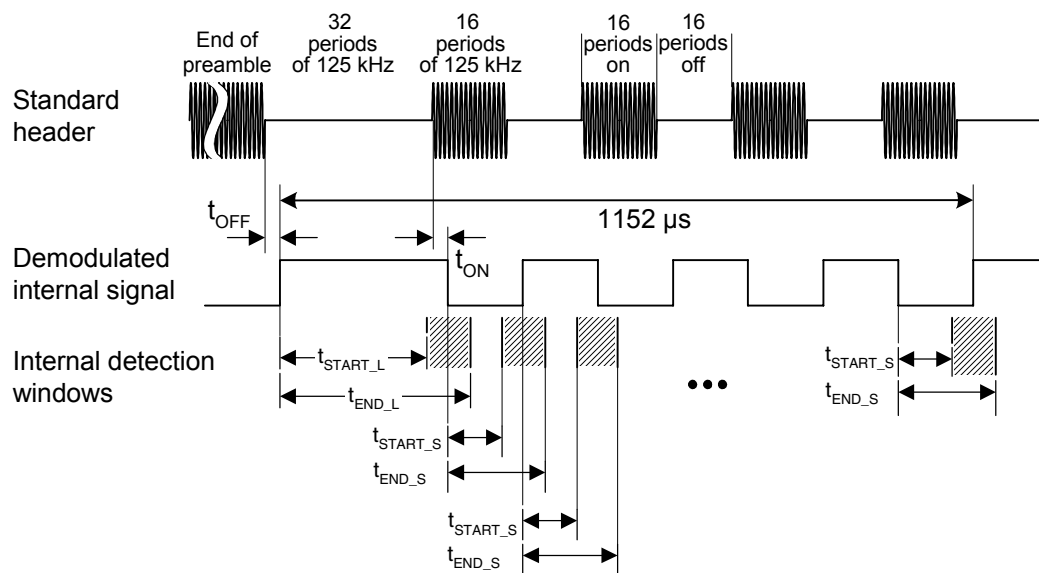
Figure 3-6. Standard Header
