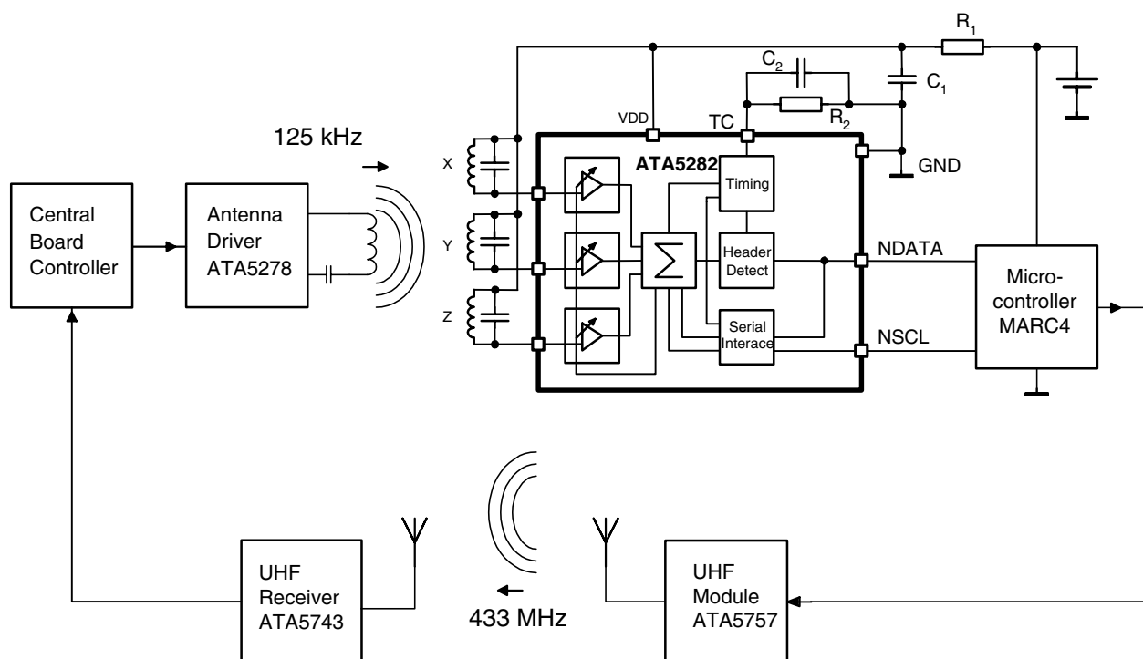
Figure 5-1. Application Circuit
