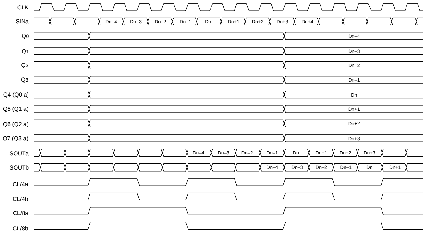
Timing Diagram
